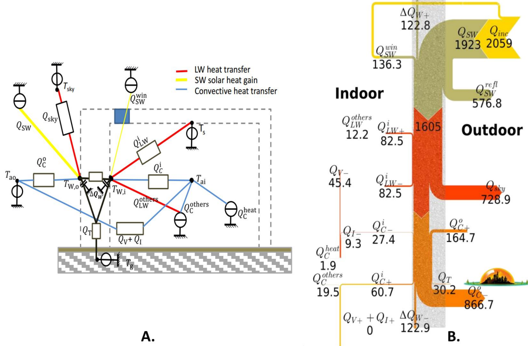
Figure 2: A. Heat transfer in the building and between the building and its environment; B. Sankey diagram (kWh/m 2 ) of the entire year
