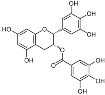
Epigallocatechin-3-gallate
