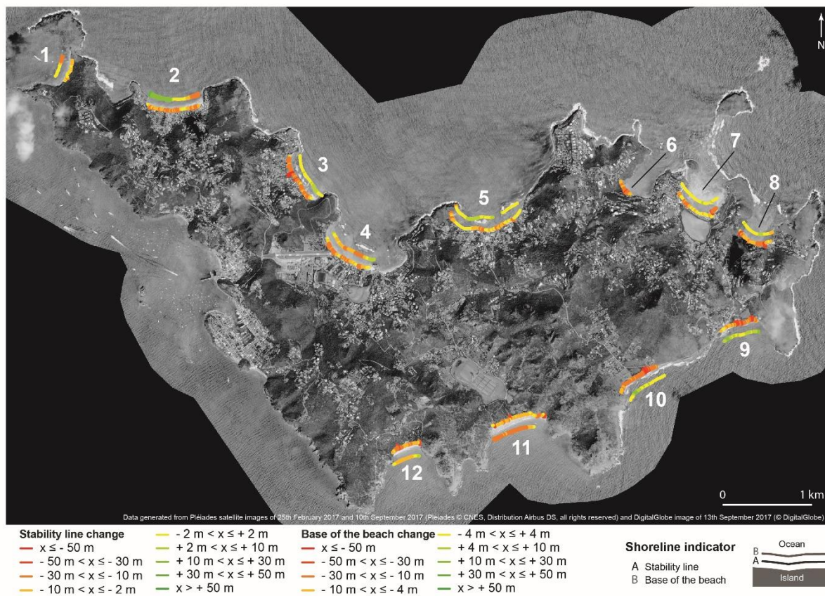
Figure 7 – Inferred impacts of September 2017 hurricanes on shoreline position on Saint-Barthélemy Island. This figure highlights first, the spatial variability of the stability line response on the island scale, depending on site exposure to the hurricane waves, and second, the contrasting behaviours of the stability line (predominantly showing retreat) and of the base of the beach (mainly exhibiting either stability, or retreat).
