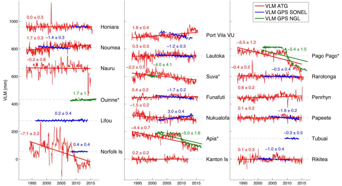
Figure 4. VLM_{ATG} time-series at tide gauge locations from the AVISO satellite altimetry database (red lines). VLM_{GPS} time-series from SONE (blue lines) and from NGL (green lines). Units are millimetres. VLM_{ATG} , VLM_{GPS} and standard error values are shown together with their corresponding linear trend lines (units in mm/year). Asterisks denote the locations where robust VLM_{GPS} trends from SONE are not available and VLM_{GPS} time-series, in this case the trends from NGL are plotted. VLM_{GPS} values are absent at the locations where robust VLM_{GPS} estimates are not available for both SONE and NGL.
