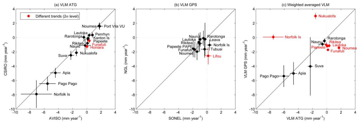
Figure 3. Scatterplot between trends of vertical land motion from (a) satellite radar altimetry minus tide gauge (VLM ATG ) data from AVISO and CSIRO, (b) GPS data from SONEL and NGL, and (c) weighted means of VLM ATG and VLM GPS trends (see section 3). Error bars denote one \sigma standard error. In red colour denotes that trends are different at the 2 \sigma significance level (T-test).
