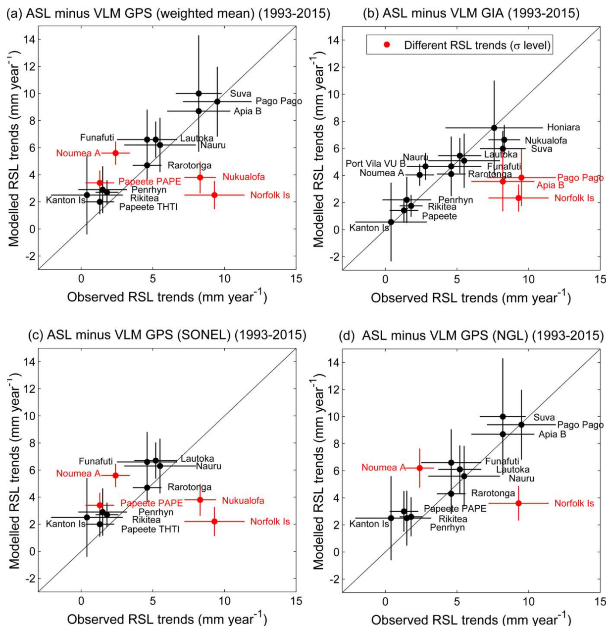
Figure S5. Scatterplot between observed and modelled RSL trends obtained from ASL trends (AVISO) minus vertical land motion trends from weighted mean VLM_{GPS} trends (a), VLM_{GIA} trends (b) and VLM_{GPS} trends from SONEL (c) and NGL (d). Error bars denote one \sigma standard error of the trends. Red dots and bars denote different trends at \sigma significance level (T-test).
