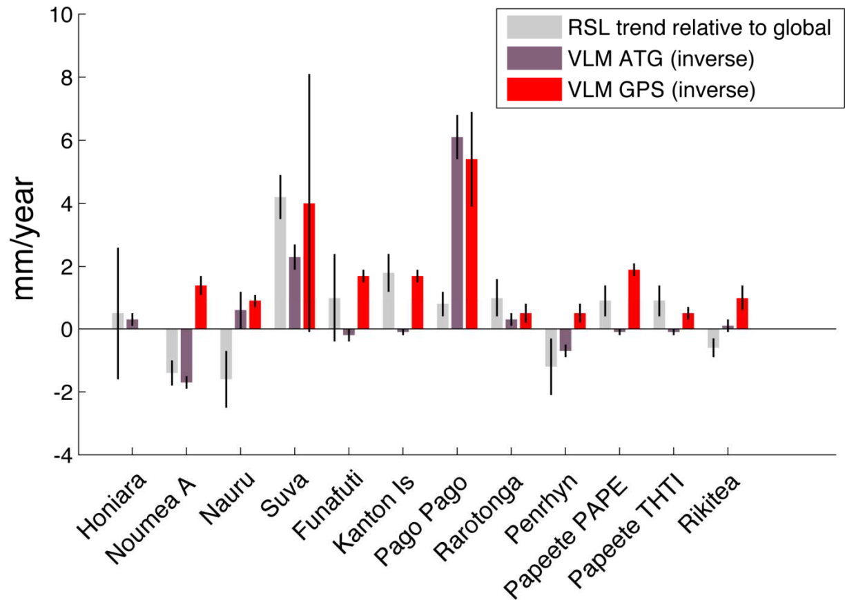
Figure S4. Difference between local RSL trends and global mean sea-level rise (mm/year) at the longest tide gauges (light grey bars). Inverse of the vertical land motion rate (mm/year) obtained from weighted averaged VLM_{ATG} (purple bars) and VLM_{GPS} (red bars). Error bars (vertical black lines) denote standard errors.
