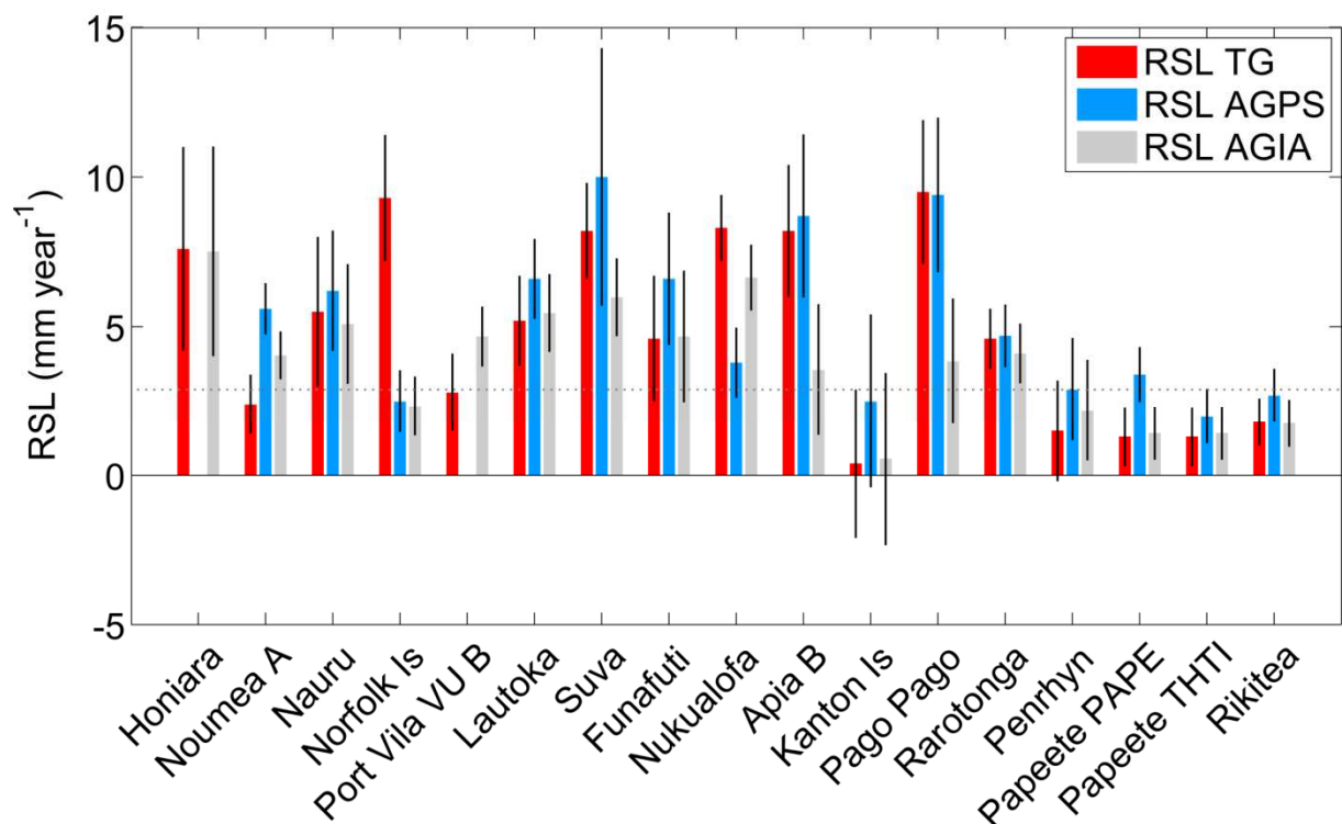
Figure S3. RSL TG: Trends of relative sea level from tide gauges records (red bars), satellite radar altimetry (AVISO) minus weighted averaged VLM_{GPS} trends (blue bars) and satellite radar altimetry (AVISO) minus modelled VLM_{GIA} (grey bars). Error bars denote one standard error of the trends.
