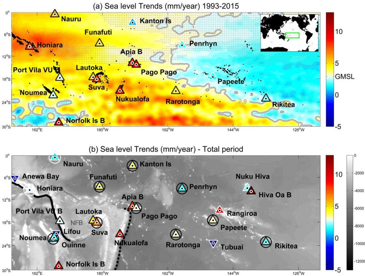
Figure 1. Relative Sea level trends (mm/year) at tide gauges (coloured triangles) and absolute sea level trends at AVISO altimetry grid points (coloured areas) calculated over the 1993-2015 period (a) and over the total period of each tide gauge (b). Grey contours mark global
