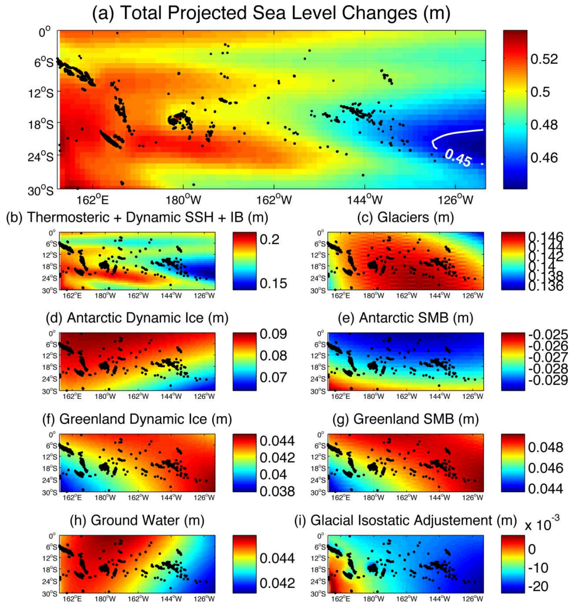
Figure S1. Regional sea-level changes of the different sea level contributions from RCP8.5 over the period from 1986–2005 to 2081–2100 (in meters). Total projected regional sea-level changes resulting from the sum of all the contributions (a). The CMIP5-RCP8.5 ensemble mean of the sum of the thermosteric, dynamic and atmospheric (b), glacier (c), ice sheet (d-g), groundwater (h) and GIA (i) contributions.
