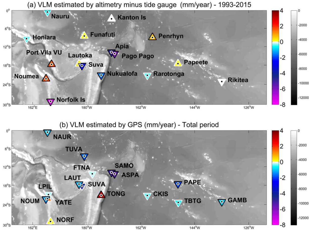
Figure 2. VLM_{ATG} weighted means (AVISO and CSIRO) calculated over 1993-2015 at the tide gauge locations (a) and VLM_{GPS} weighted means (SONEL and NGL) calculated at their closest GPS stations (b). Upward (downward) triangles denote positive (negative) VLM values. White-bordered triangles denote no statistical significance at 2\sigma level. GEBCO bathymetry (in meters) is also shown.
