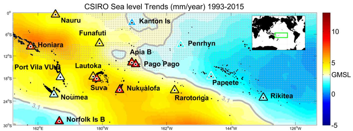
Figure S2. Sea level trends (mm/year) at tide gauges (coloured triangles) and CSIRO altimetry grid points (coloured areas) calculated over 1993-2015. Grey contours mark global mean sea level trend during 1993-2015. White-bordered triangles and dot-shaded areas denote no statistical significance at 2\sigma level.
