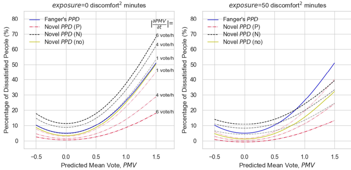
Figure 6 Predicted percentage of dissatisfied occupants as a function of PMV at different combinations of exposure (0 and 50 discomfort 2 minutes) and \left| \frac{\partial PMV}{\partial t} \right| (1, 4 and 6 vote/h) for the cases of positive (red), negative (black) and no (yellow) alliesthesia. Fanger's PPD is plotted in blue for purposes of comparison.
