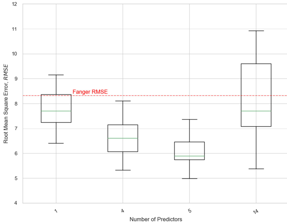
Figure 5 Boxplots of the RMSEs associated to the four different models tested. Fanger's RMSE is calculated using the entire dataset and is shown with the red dashed line.
