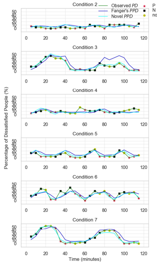
Figure 7 Percentage of dissatisfied people (observed PD, Fanger's PPD and Novel PPD) for the 6 cyclical temperature variations (conditions 2-7). The three levels of positive (P), negative (N) and no alliesthesia are highlighted in red, black and yellow respectively.
