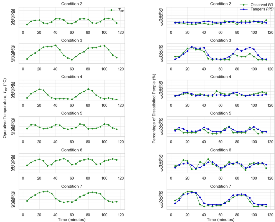
Figure 2 Operative temperature ( T_{op} , left) and percentage of dissatisfied people (observed PD and Fanger's PPD, right) for the 6 cyclical temperature variations (conditions 2-7). The observed PD represents the vote of all participating students every 5 minutes, while T_{op} corresponds to the mean calculated value every 5 minutes. Adapted from [31].
