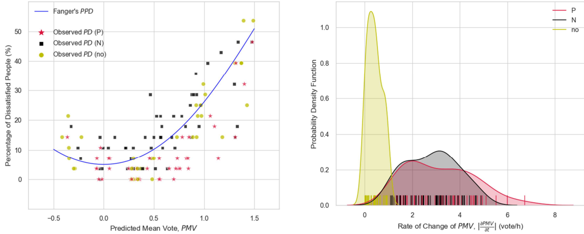
Figure 3 On the left: Observed PD as a function of PMV for the three levels of positive (P), negative (N) and no alliesthesia in red, black and yellow respectively. Fanger's PPD model is plotted in blue for purposes of comparison. On the right: Gaussian kernel density estimate of the absolute values of the rate of change of PMV.
