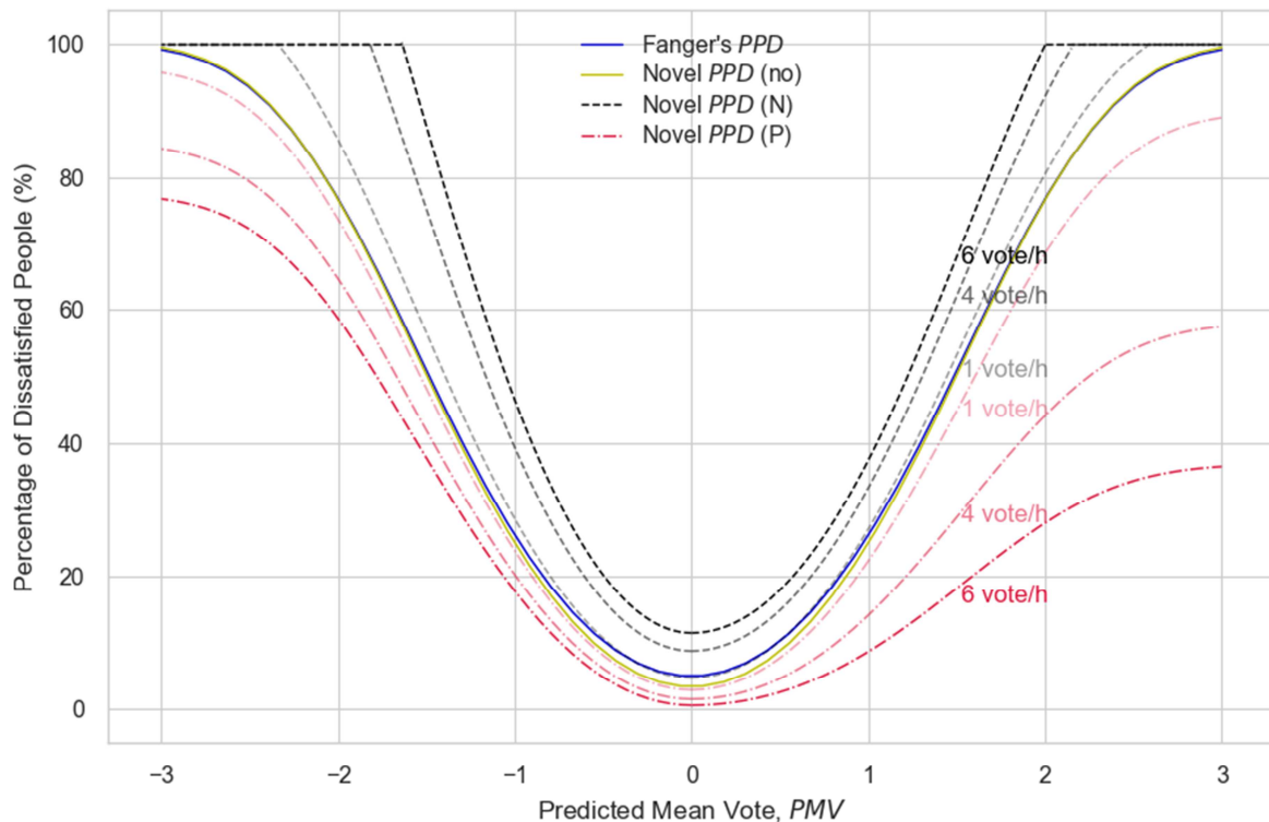
Figure 9 Extended novel PPD model for exposure equal to 0 discomfort 2 minutes.
