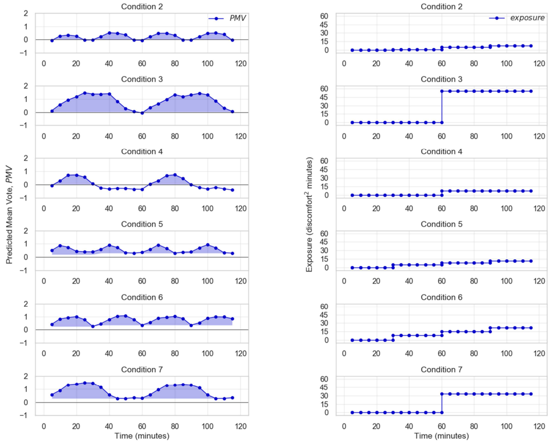
Figure 4 Calculated PMV (left) and exposure (right) for the 6 cyclical temperature variations (conditions 2-7).
