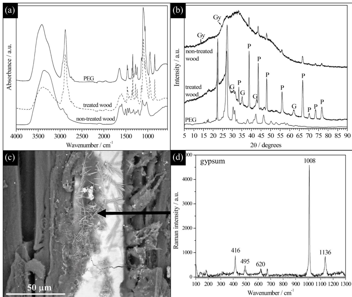
Figure 7: FTIR spectra (a) and XRD patterns (b) of non-treated wood, treated wood and PEG used for treatment. ESEM micrograph of a non-treated sample (c), Raman spectrum of gypsum (d). P = pyrite, G = greigite, Gy = gypsum.
