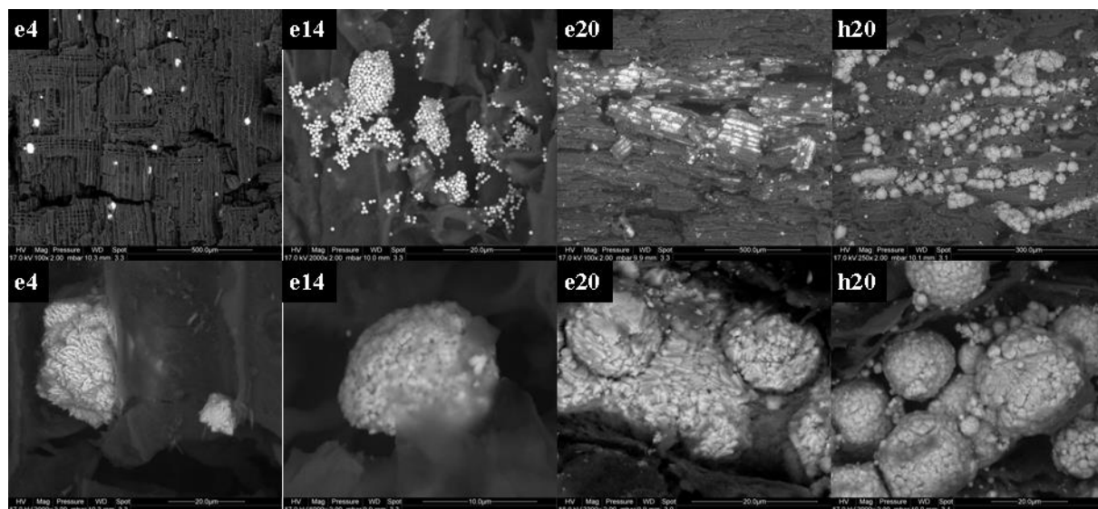
Figure 5. ESEM micrographs of e4, e14, e20, h20 samples
