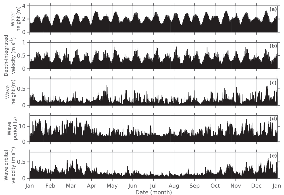
Figure 4. Time series of the 2012 simulated (a) water height, (b) depth-integrated velocity, (c) significant wave height, (d) wave period of the second moment, and (e) wave orbital velocity.
