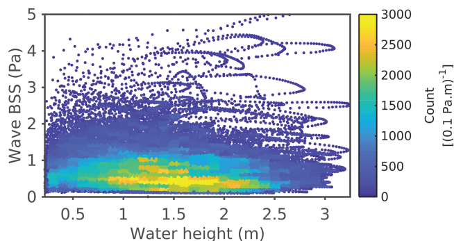
Figure 12. Relationship between the simulated wave BSS and the water depth.
