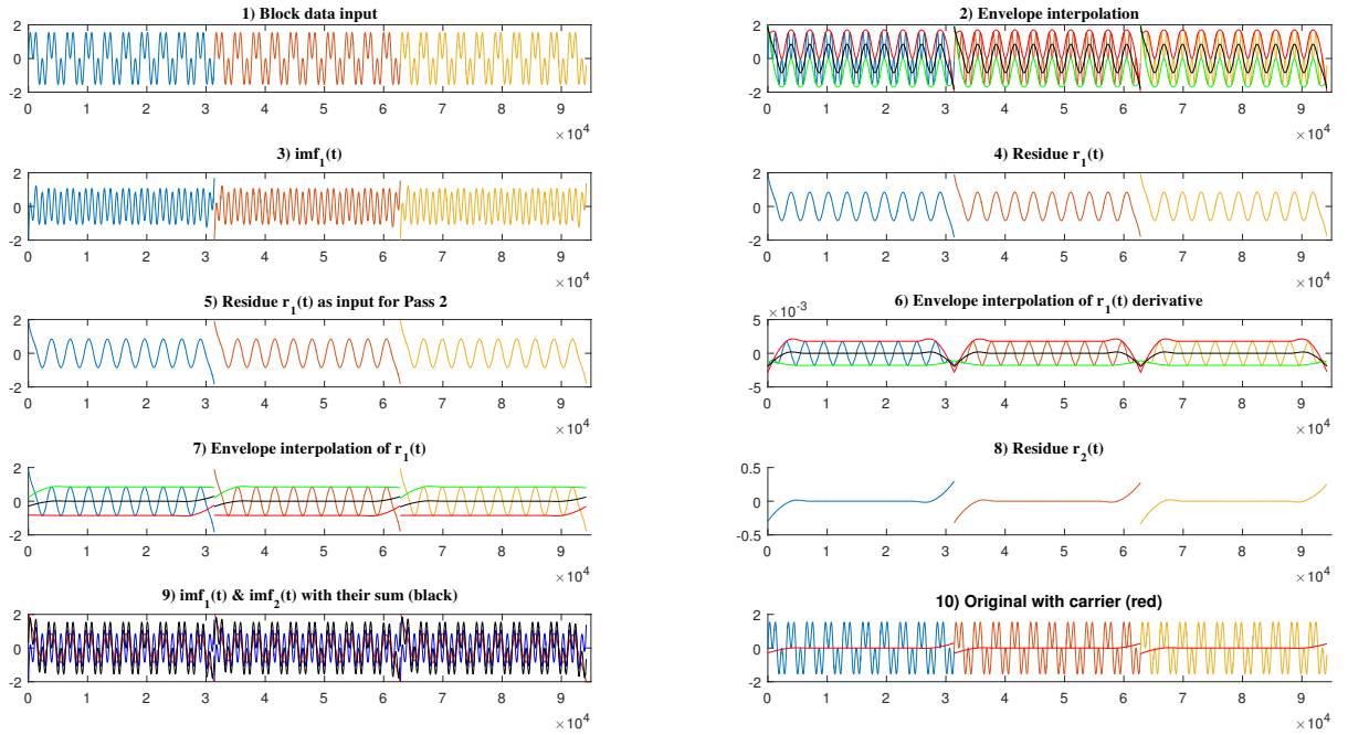
Figure 6: on-line SWEMD without elimination of the end effect.
