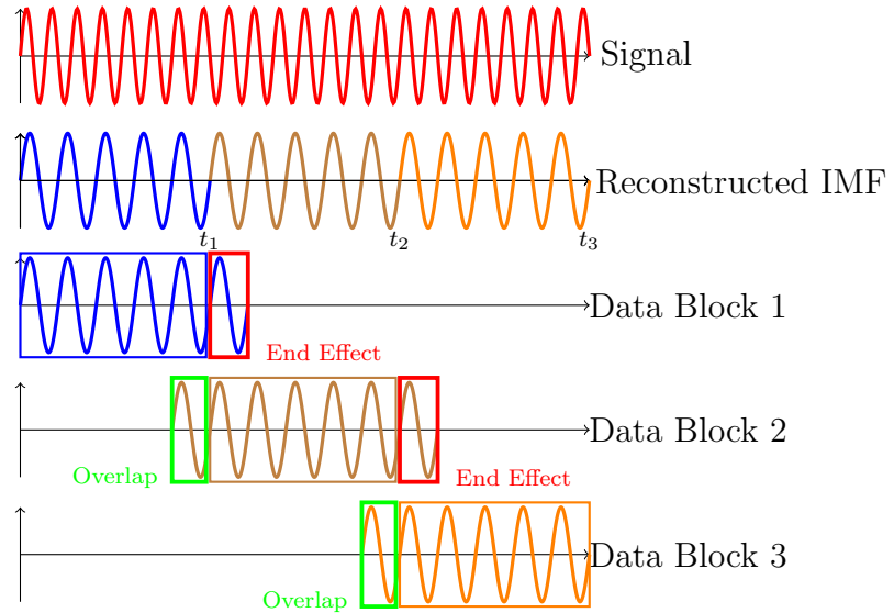
Figure 7: End effect elimination illustrative example in blockwise (windowed) EMD.
