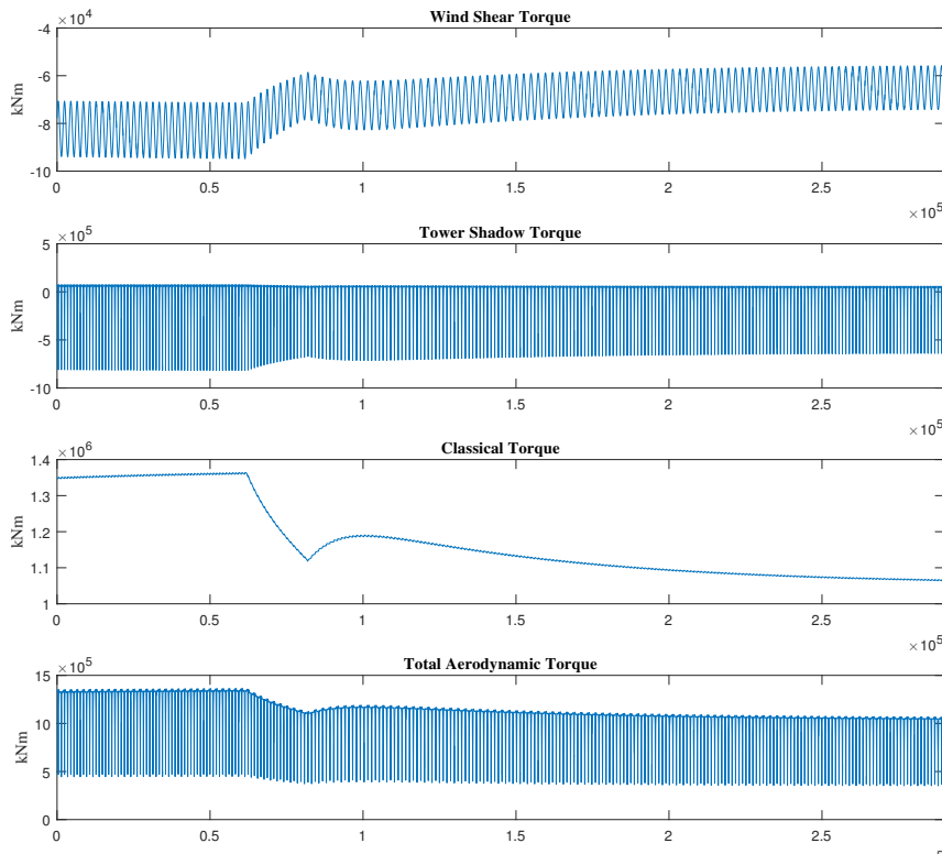
Figure 11: Aerodynamic torque produced by the wind profile.
