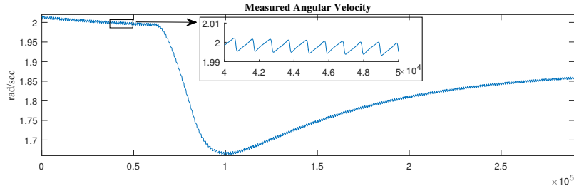
Figure 12: Turbine side angular velocity.
