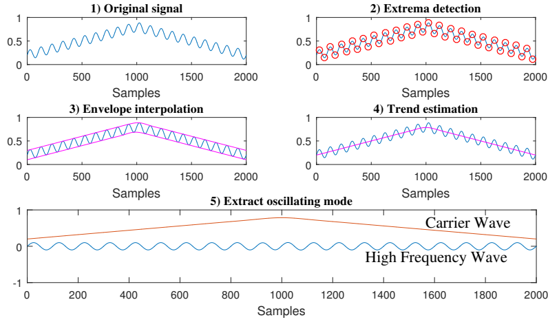
Figure 3: EMD methodology representation.
