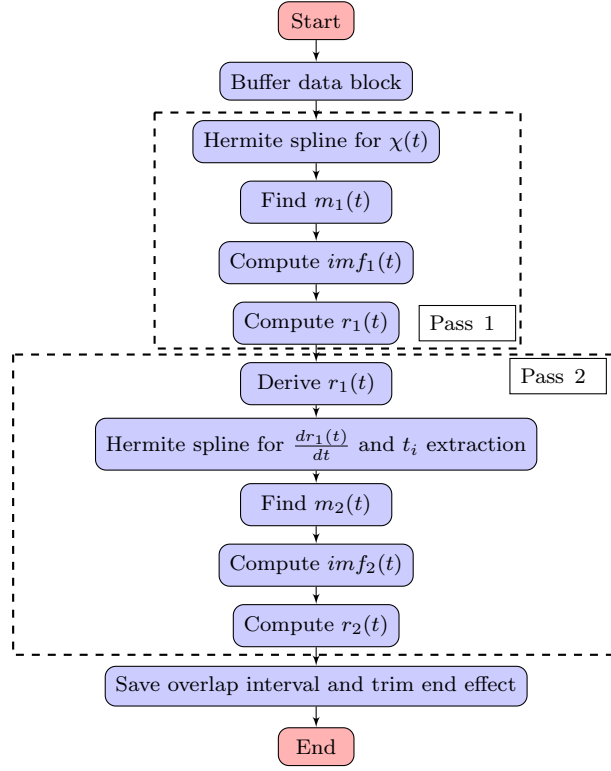
Figure 5: Flowchart for EMD harmonic isolation.
