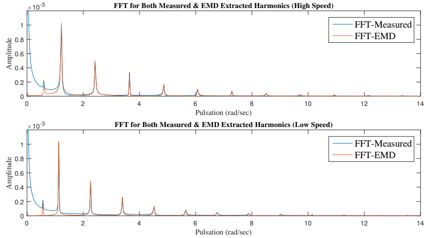
Figure 15: FFT comparison between the original signal and its extracted harmonics through EMD (High speed section on top, Low speed section at the bottom).
