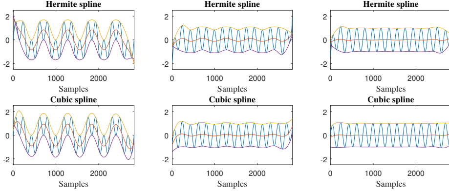
Figure 4: Hermite (top) versus Cubic (bottom) interpolation for three IMF extraction iterations.
