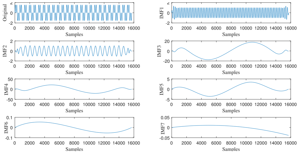
Figure 2: EMD decomposition of \chi(t) = x_1(t) + x_2(t) .
