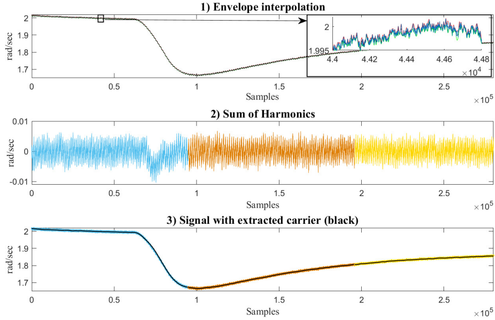
Figure 16: Modified EMD for the turbine side angular velocity measurement with added pink noise.
