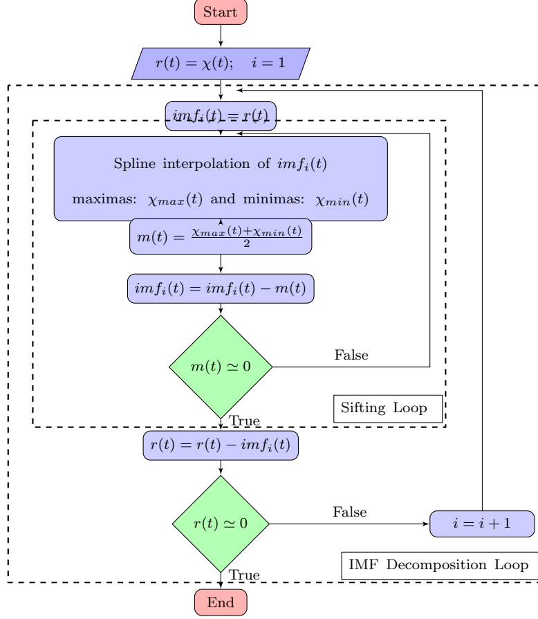
Figure 1: Flowchart for EMD algorithm.
