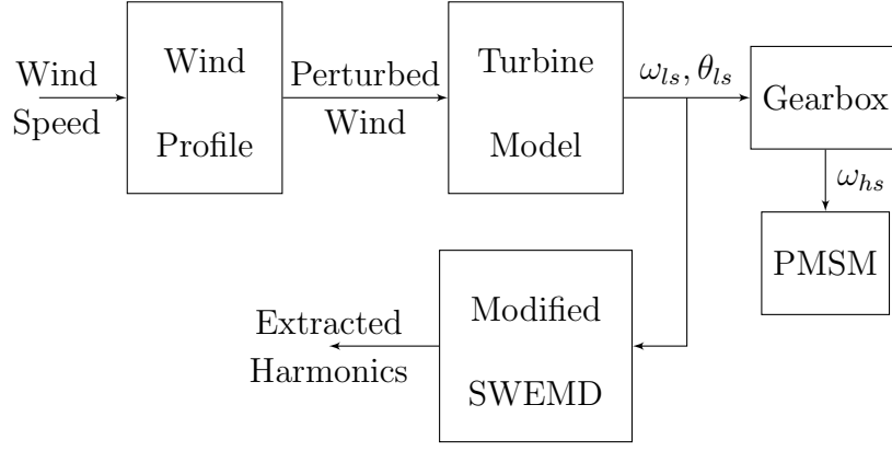
Figure 13: Bloc Diagram of the modified SWEMD harmonics extraction for angular velocity signal.
