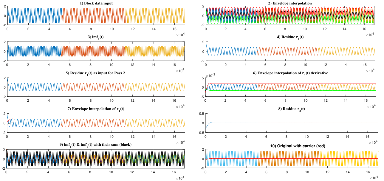
Figure 8: on-line SWEMD with elimination of the end effect.
