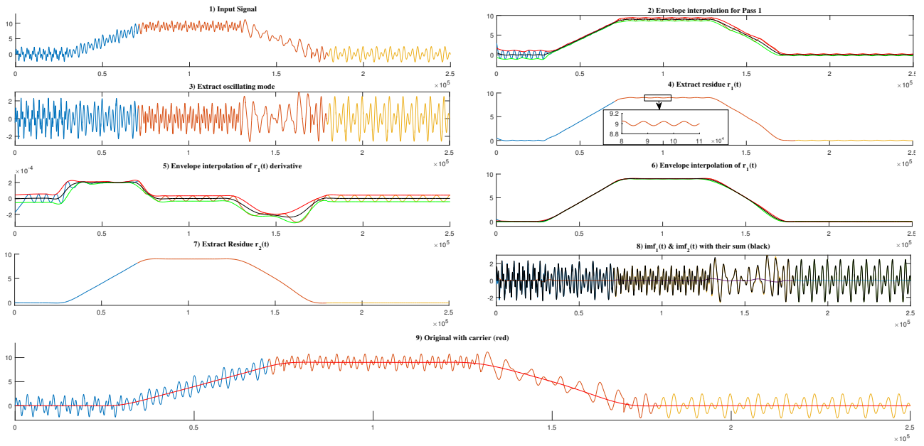
Figure 10: Modified SWEMD applied to a non-stationary signal.
