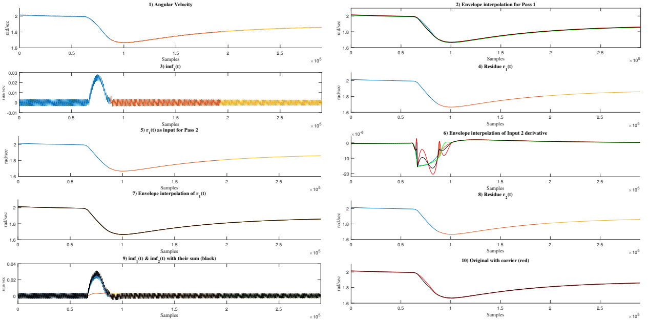
Figure 14: modified SWEMD applied for angular velocity harmonics extraction.
