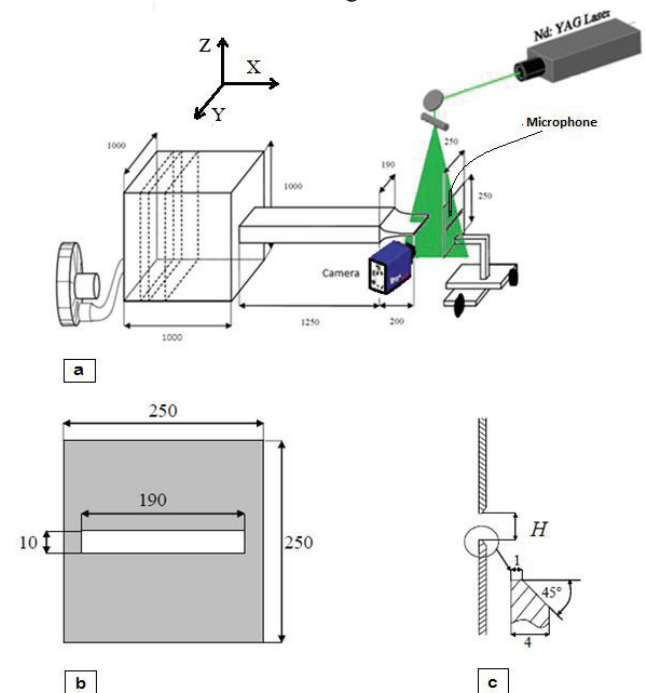
Figure 1. Dispositif exp rimental
