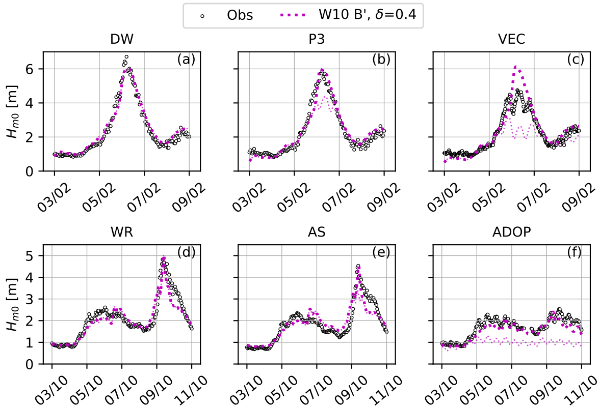
Figure 10: Measured and simulated H_{m0} for the two study cases using W10 formulation with a modified parameterization of the biphasic. The thin light grey curves correspond to the results obtained with the default parameterization
