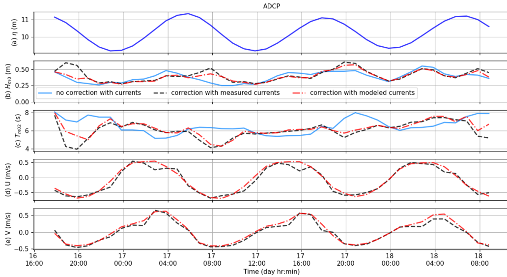
Figure A1. (a) Water elevations measured at the ADCP station (see location on Figure 1b). Temporal series of H_{m0} (b) and T_{m02} (c) obtained without current effect (solid line), or by including measured (dashed line) or modelled (dashed-dotted line) currents in the wave dispersion relation, with the corresponding zonal ( U ) and meridional ( V ) components of currents illustrated on (d) and (e), respectively.
