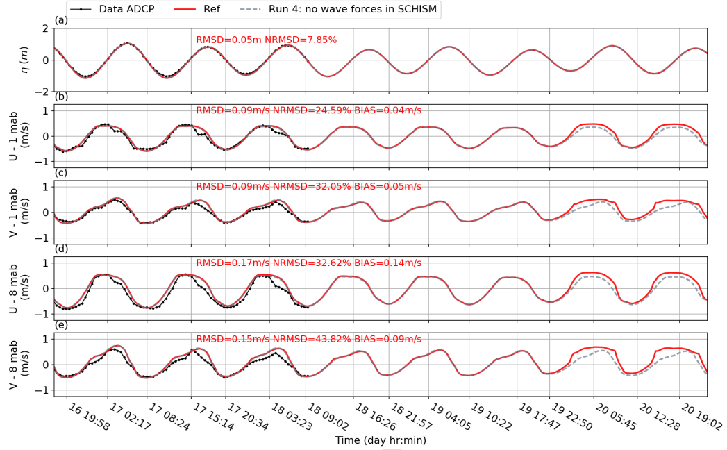
Figure 6. Comparisons of ADCP data and model results from simulations Ref and Run 4 (no wave forces in SCHISM) in terms of sea surface elevation (a; around mean sea level), and zonal ( U ) and meridional ( V ) components of currents at 1 m above the bed (on b and c, respectively) and 8 m above the bed (on d and e, respectively). Statistical parameters RMSD, NRMSD and BIAS refer to the Ref accuracy with respect to observations.
