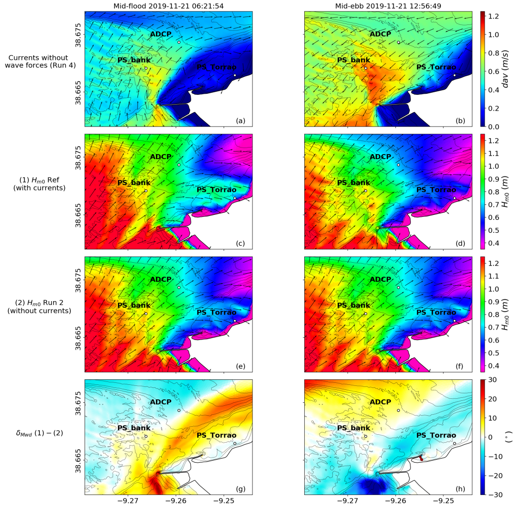
Figure 11. Spatial distributions of depth-averaged currents, dav , at successive mid-flood (a) and mid-ebb (b) situations during the storm peak and the corresponding fields of significant wave height, H_{m0} , from simulations (1) Ref (with currents) and (2) Run 2 (without currents) at mid-flood, (on (c) and (e), respectively), and at mid-ebb, (on (d) and (f), respectively) (see the corresponding thick vertical ticks associated with these specific dates on Figure 5). Changes in the mean wave direction between Run 2 and Ref (1-2) are illustrated at mid-flood and mid-ebb on (g) and (h), respectively.
