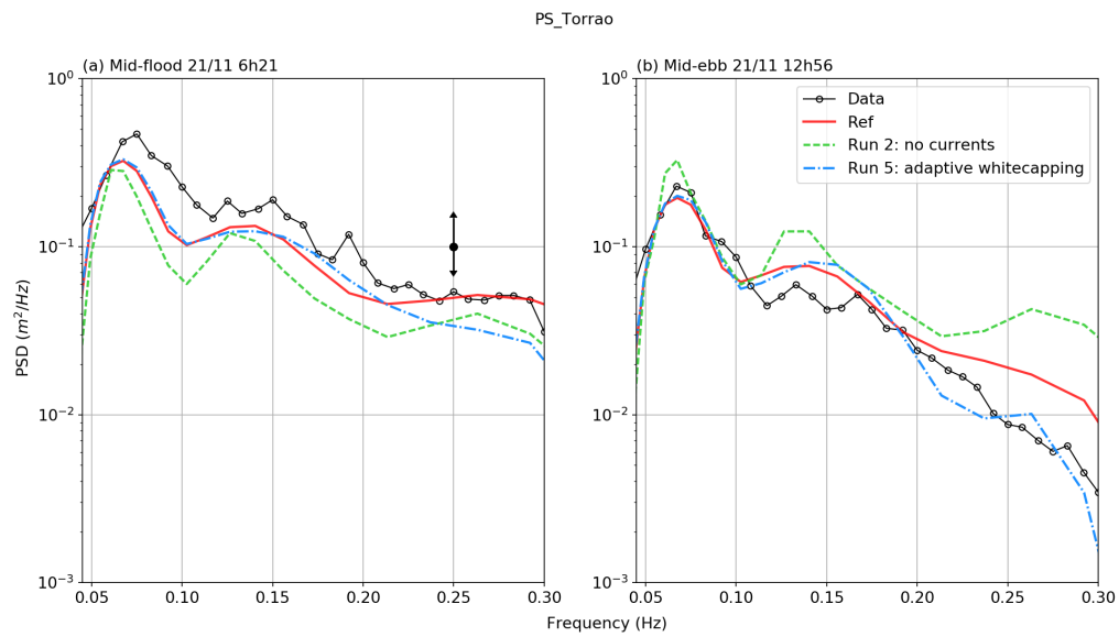
Figure 10. Power spectral density (PSD) obtained from pressure measurements, and simulations Ref , Run 2 (no currents) and Run 5 (adaptive whitecapping) at PS_Torrao during successive mid-flood (a) and mid-ebb (b) situations, the 21 st of November at 6:21 and 12:56, respectively (see the corresponding thick vertical ticks on Figure 5).
