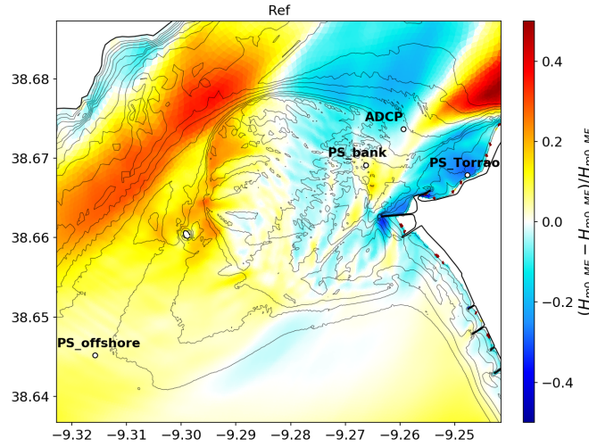
Figure 12. Increasing/decreasing trends of the significant wave height, H_{m0} , between two successive mid-flood (MF, 20 th November at 5:02am) and mid-ebb (ME, 20 th November at 11:46am) situations during the storm peak, obtained from simulation Ref . Trends are expressed as (H_{m0,ME} - H_{m0,MF})/H_{m0,MF} , a positive value meaning that H_{m0} increases at ME, and vice versa.
