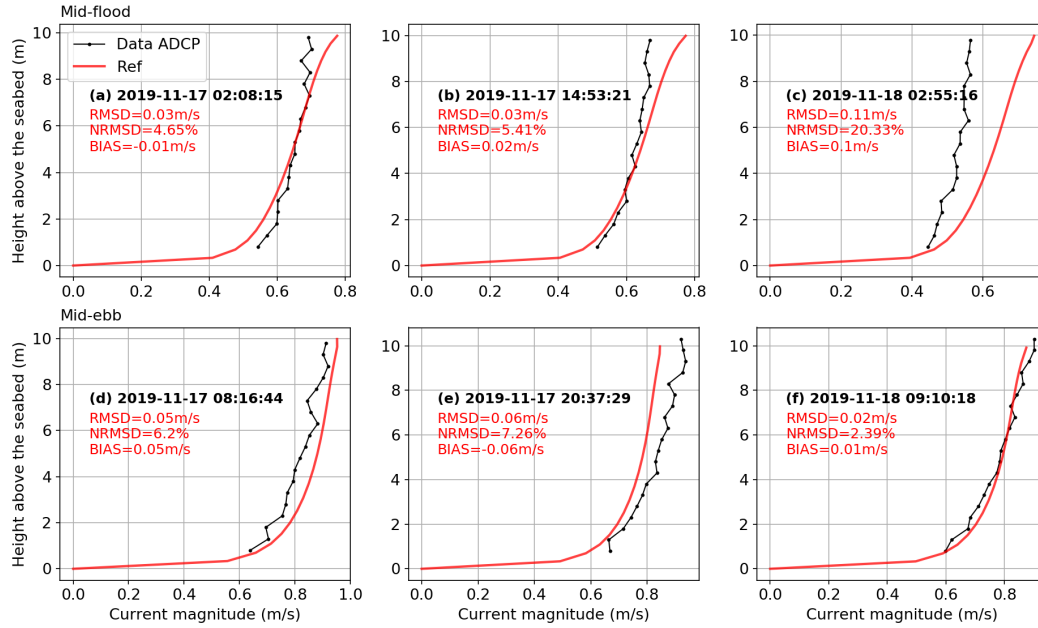
Figure 7. Comparisons of vertical profiles of currents (magnitude) obtained from the ADCP data and model results from simulation Ref , at 3 mid-flood (from a to c ) and 3 mid-ebb situations (from d to f ). Statistical parameters RMSD, NRMSD and BIAS refer to the Ref accuracy with respect to observations.
