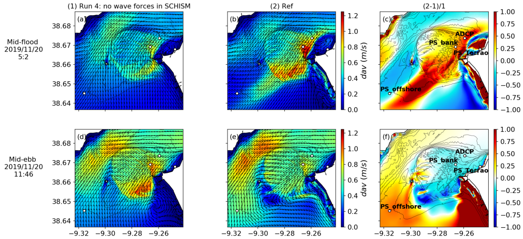
Figure 13. Spatial distributions of depth-averaged currents, d_{av} in m/s, at successive mid-flood (MF) and mid-ebb (ME) situations during the storm peak, obtained from simulations (1) Run 4 [no wave forces in SCHISM] (on (a) and (d), respectively) and (2) Ref (on (b) and (e), respectively). The increasing/decreasing trends of d_{av} between Run 4 and Ref at MF and ME [(2-1)/1] are illustrated on (c) and (f), respectively.
