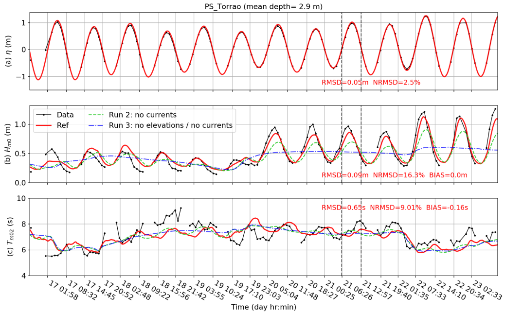
Figure 5. Comparisons of sea surface elevation (a), significant wave height H_{m0} (b), and mean wave period T_{m02} (c) at PS_Torrao station (see location on Figure 1b) between data and model results from simulations Ref , Run 2 (no currents) and Run 3 (no elevations and no currents). RMSD, NRMSD and BIAS values indicated on each subplot refer to simulation Ref . Thicker vertical ticks refer to specific dates used in the following analyses.
