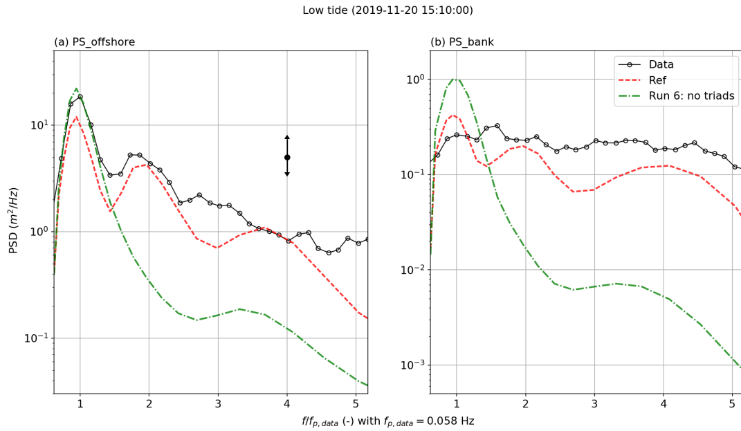
Figure 9. Power spectral density (PSD) as a function of normalized frequency (by f_{p,data}=0.058 Hz) obtained from pressure measurements, and simulations Ref and Run 6 at PS_offshore (a) and PS_bank (b) during a low tide situation occurring at the storm peak (the 20 th of November at 3:10pm). On (a), the error bar refers to the 95% interval of confidence of the PSD (Bendat and Piersol, 1971).
