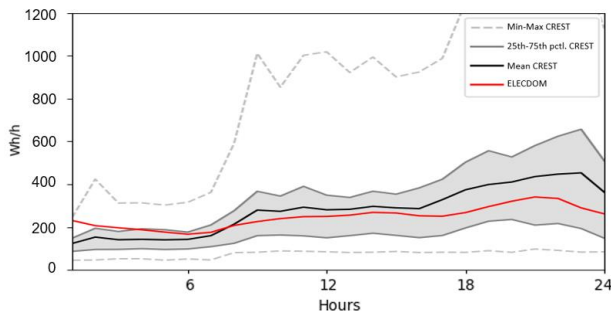
Figure 2: Comparison of a mean daily load profile modelled with CREST with measured data (ADEME, 2021)
