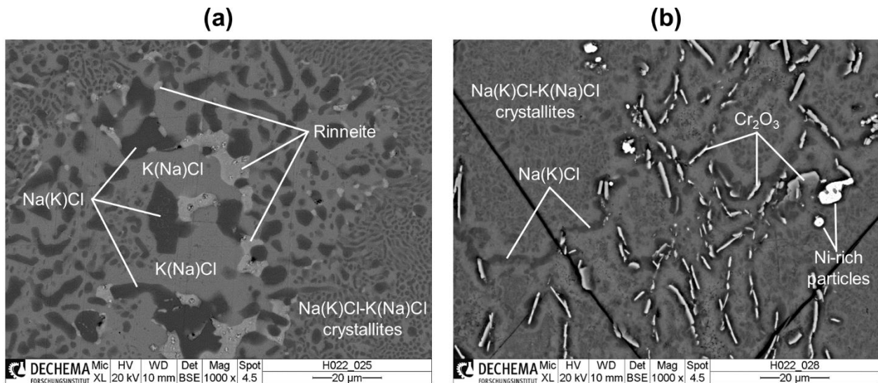
Fig. 4. BSE cross-section images of the residual salt mixtures taken in representative areas after exposure of (a) P91 and (b) Inconel 600 to molten NaCl-KCl at 700^\circ\text{C} in flowing Ar for 300 h.
