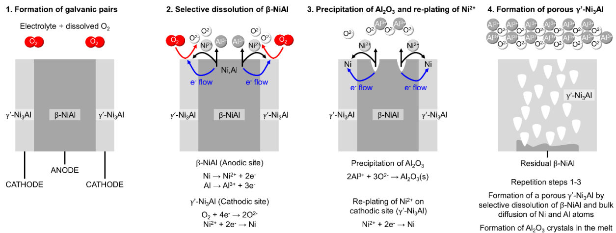
Fig. 14. Schematic illustration of the galvanic corrosion process of \beta\text{-NiAl} resulting in the formation of a porous \gamma\text{-Ni}_3\text{Al} coating layer and non-protective \text{Al}_2\text{O}_3 crystals above the coating surface. \text{Ni}_5\text{Al}_3 phase was not considered to simplify the mechanisms but a similar process may be expected between \text{Ni}_5\text{Al}_3 (anode) and \gamma\text{-Ni}_3\text{Al} (cathode). Unlike dezincification of brass alloys and dealuminification of aluminium bronze alloys in aqueous solutions, solid-state diffusion mechanisms play a major role in the corrosion mechanisms such that phase transformation may trigger the attack.
