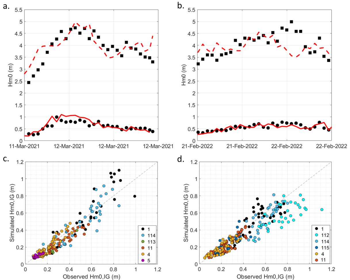
Figure 5 : Observed vs simulated wave parameters: Time series of observed (black symbols) and modeled (red lines) wave bulk parameters at the location of Pt 1 sensor (Figure 1a), H_{m0, SW} (black squares vs red dashed line) and H_{m0, IG} (black circle vs red solid line) for the storms 2021 (a) and 2022 (b); (c-d) Observed vs Modeled H_{m0, IG} , with all sensors for the storms 2021 (c) and 2022 (d).
