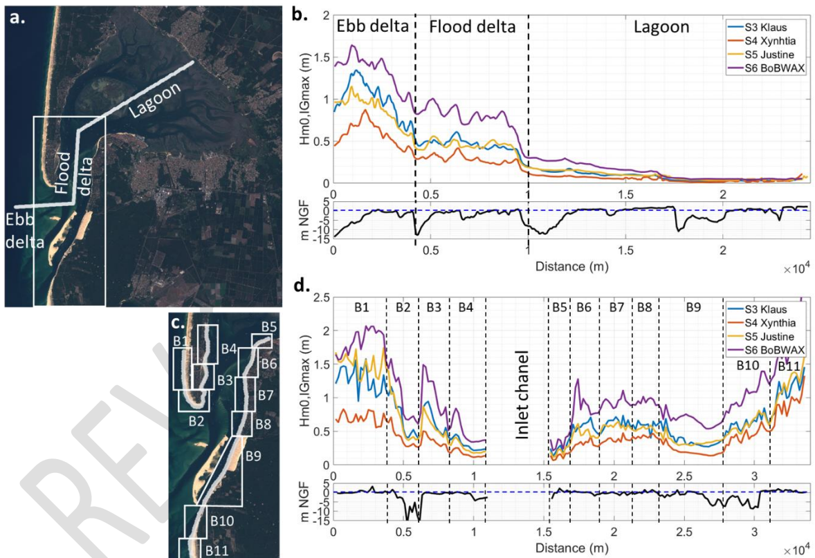
Figure 10 : Simulated IG wave significant wave height peak along the inlet at the coast for historical and extreme storm conditions: a) location of cross inlet-lagoon transect b) H_{m0}, IG_{max} and bathymetry profile, c) delimitation of coastal segment at the inlet, d) H_{m0}, IG_{max} at the inlet coast.
