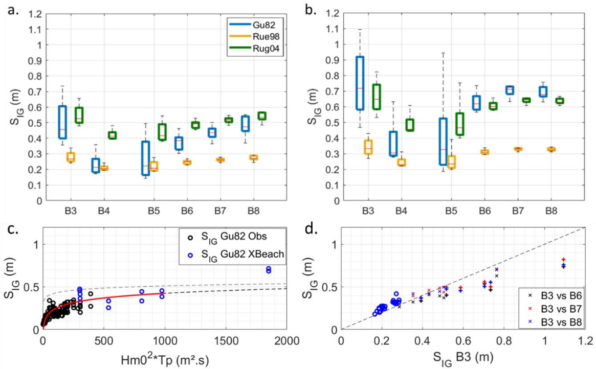
Figure 13 : Wave induced swash ( S_{IG} ) estimates for a.) S1 (common winter storm) and b.) S6 (statistical extreme storm) with the formulation : S_{IG} = 0.71H_{m0} + 0.035 (Guza and Thornton, 1982, noted Gu82); S_{IG} = 0.18H_{m0} + 0.16 (Ruessink et al., 1998) ; S_{IG} = 0.33H_{m0} + 0.33 (Ruggiero et al., 2004, noted Rug04) along the coast of the inlet, (refer to Figure 9 for the delimitation of the coastal segment). The subplot c.) illustrates the relation between the offshore wave energy H_{m0}^2 * T_p and the S_{IG} based on the Gu82 estimator. Circles represents observations at Pt 11 and Pt4 (dark) and alongshore-average simulated (blue) values for B3 and B8. The red solid curve prolonged by the black dashed line is the log regression associated to the Gu82 estimator for alongshore-averaged S_{IG} . The grey curve is the log regression associated to the Ru4 estimator. The subplot d.) illustrates the relation between S_{IG} at wave exposed shore of the inlet (B6, B7, B8) with respect to the sheltered part of the inlet (B3). Circles, thin (x) and bold (+) crosses represent observations, alongshore-averaged and alongshore-maximum values respectively.
