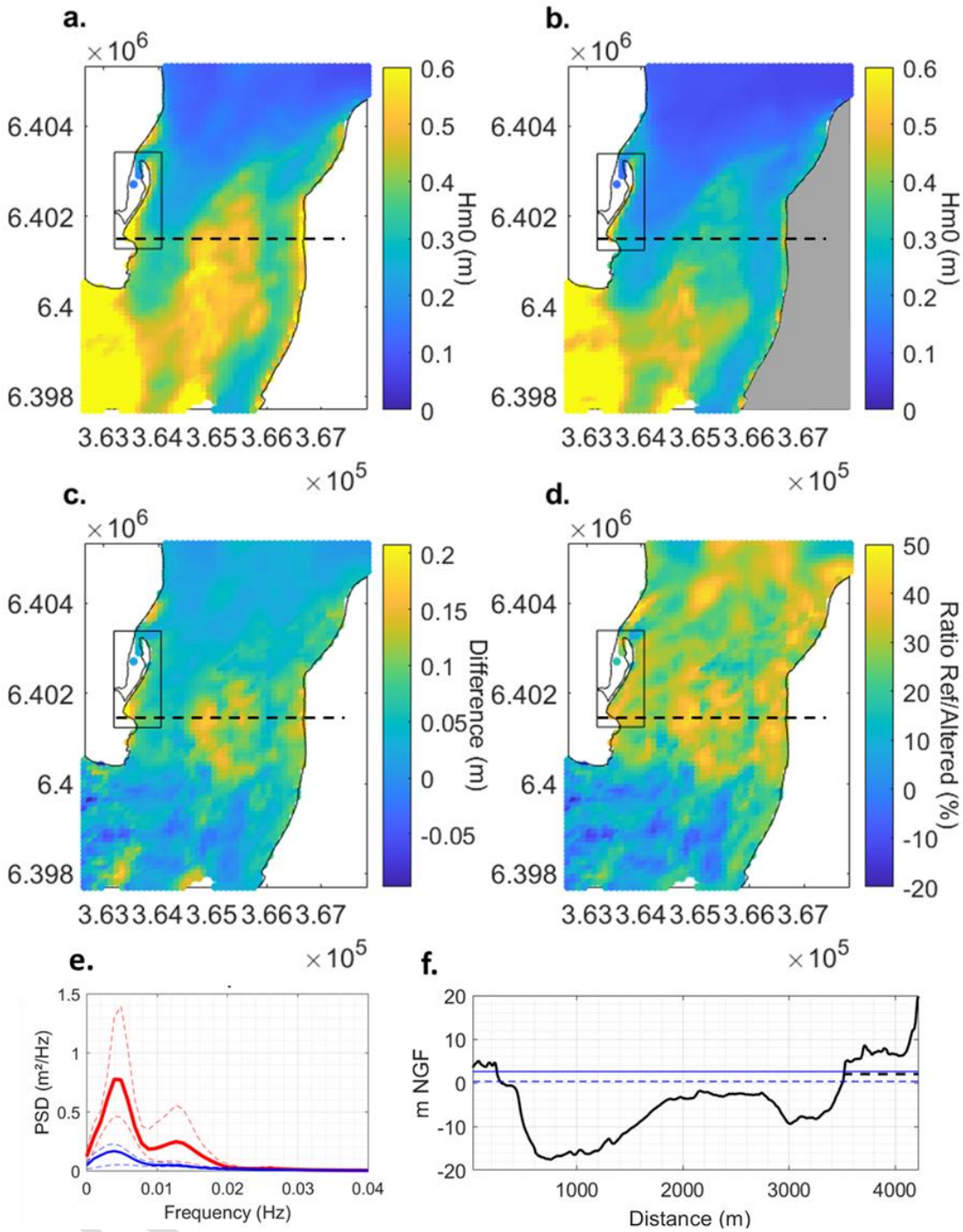
Figure 12 : H_{m0,IG_{max}} at internal part of the inlet for S1 storm with a.) the reference bathymetry, b.) the altered bathymetry (modification of the wave-exposed coast topo-bathymetry (the grey area), c.) H_{m0,IG_{max}} difference, d.) ratio between the difference and the original simulation, e. IG wave energy density spectra at the proximal end (Pt 4 locations) of the Mimbeau Spit (black rectangle). The red and the blue curves represent the time-averaged spectra during high tide (2 h) on the reference and the altered bathymetry, respectively. Dashed lines represent the 95% confidence interval. f.) illustrate the topobathymetric cross-channel profile (along the dashed line in a., b., c., d. subplot), black solid and dashed lines illustrate the reference and the altered topo-bathymetry, respectively. The blue solid and dashed lines, high tide water level (2.5 m NGF) and the mean sea level, respectively.
