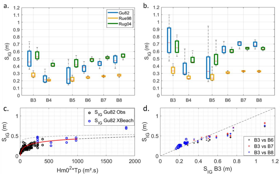
Figure 13 : Wave induced swash ( S_{IG} ) estimates for a.) S1 (common winter storm) and b.) S6 (statistical extreme storm) with the formulation : S_{IG} = 0.71H_{m0} + 0.035 (Guza and Thornton, 1982, noted Gu82); S_{IG} = 0.18H_{m0} + 0.16 (Ruessink et al., 1998) ; S_{IG} = 0.33H_{m0} + 0.33 (Ruggiero et al., 2004, noted Rug04) along the coast of the inlet, (refer to Figure 9 for the delimitation of the coastal segment). The subplot c.) illustrates the relation between the offshore wave energy H_{m0}^2 * T_p and the S_{IG} based on the Gu82 estimator. Circles represents observations at Pt 11 and Pt4 (dark) and alongshore-average simulated (blue) values for B3 and B8. The red solid curve prolonged by the black dashed line is the log regression associated to the Gu82 estimator for alongshore-averaged S_{IG} . The grey curve is the log regression associated to the Ru4 estimator. The subplot d.) illustrates the relation between S_{IG} at wave exposed shore of the inlet (B6, B7, B8) with respect to the sheltered part of the inlet (B3). Circles, thin (x) and bold (+) crosses represent observations, alongshore-averaged and alongshore-maximum values respectively.
