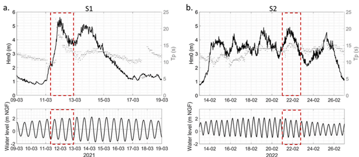
Fig. 3. Offshore storm wave time series at the Cap Ferret Buoy (observations for the 2021, 2022) and storm tide time series from the MARC operational model a) winter 2021 event and b) winter 2022 event. The red dashed rectangles bound the simulation periods for S1 and S2.
