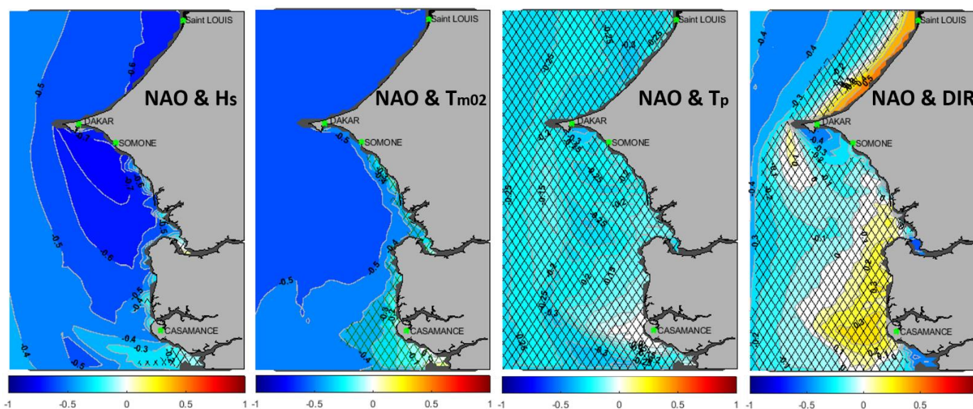
Figure 8: Spatial correlations between NAO and wave parameters (Hs, T m02 , T p , DIR) during Boreal Winter (DJFM), computed on the Senegalese coast from 1980-2021, crosslines on maps indicate areas with non-significant correlations (at 95% confidence interval from Mann Kendall Test).
