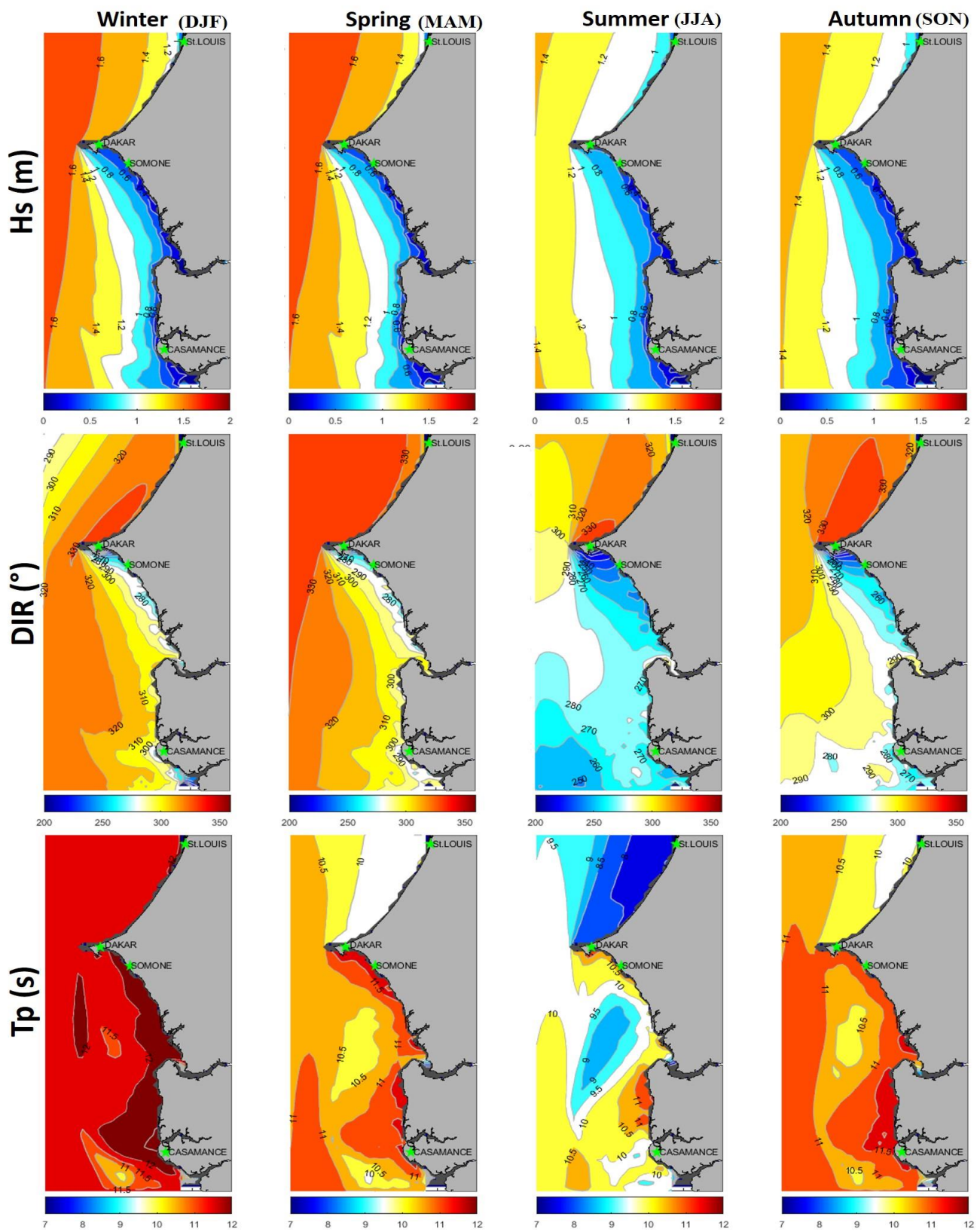
Figure 5. Spatial maps of seasonal mean wave climate: significant wave height ( H_s (m), top panel), mean wave direction ( Dir (°), at middle) and Peak period ( T_p (s), bottom panel) computed on the Senegalese Coast from 1980 to 2021. The dark grey patches along the coastline denote areas of insufficient model resolution.
