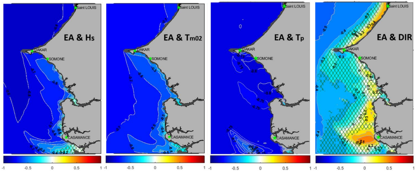
Figure 10. Spatial correlations between East Atlantic mode (EA) and wave parameters (Hs, Tm02, Tp, DIR), computed on the Senegalese coast from 1980-2016 in boreal Winter (DJF), crosslines on maps indicate areas with non-significant correlations (at 95% confidence interval, Mann Kendall Test).
