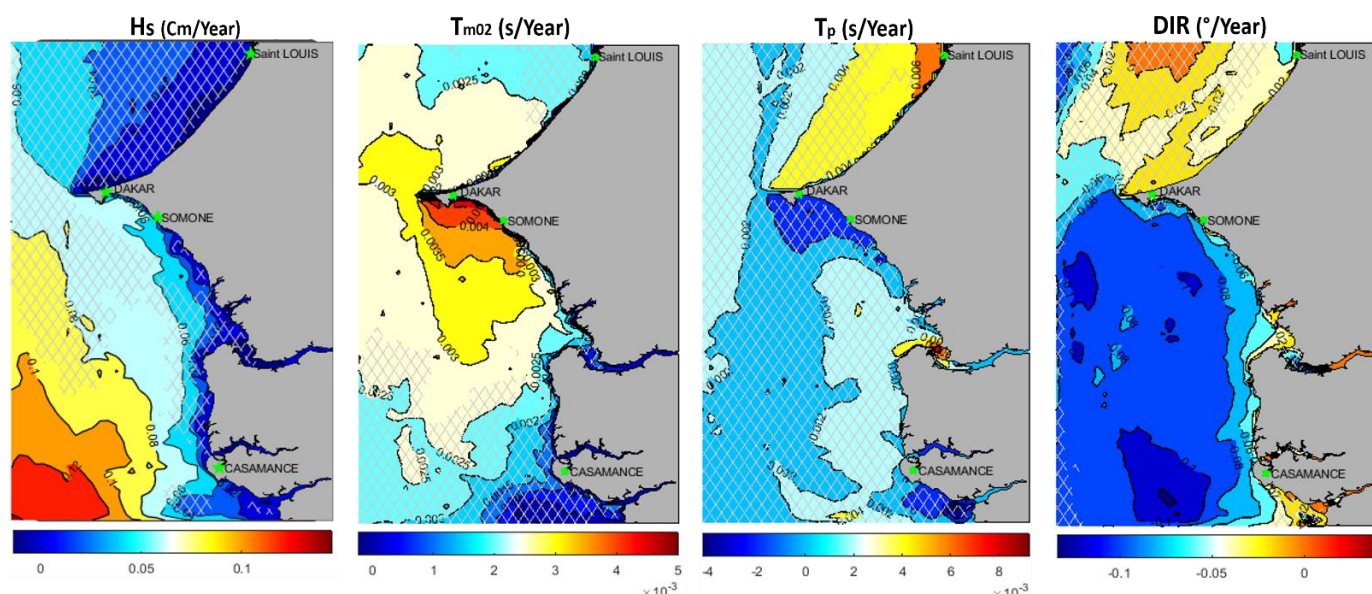
Figure 6: Trends of wave parameters (from left to right), significant wave height (Hs (cm)), wave mean period ( T_{m02} (s)), pic period ( T_p (s)) and mean direction (Dir ( ^\circ )) computed on the Senegalese Coast from 1980 to 2021, Hatched zones on maps indicate areas where trends are not significant at 95% (Mann-Kendall Test).
