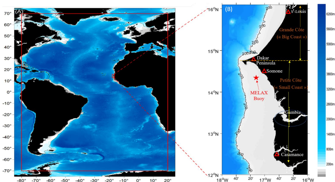
Figure 1. Atlantic Ocean Bathymetry with, (A) the extension of the regional domain grid (red rectangle) and (B) the extension of the local grid on the Senegal Coast where the Melax Buoy is referenced (red star) off Somone on the Petite Côte of Senegal.
