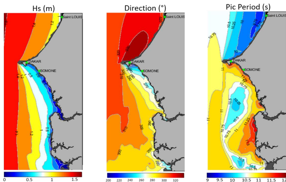
Figure 3. Spatial maps of the yearly means wave climate, significant wave height ( H_s (m), left), mean wave direction ( Dir ( ^\circ ), middle) and Pic period ( T_p (s), right) computed on the Senegalese Coast from 1980 to 2021 (Brown patches along the coastline denote areas with insufficient resolution).
