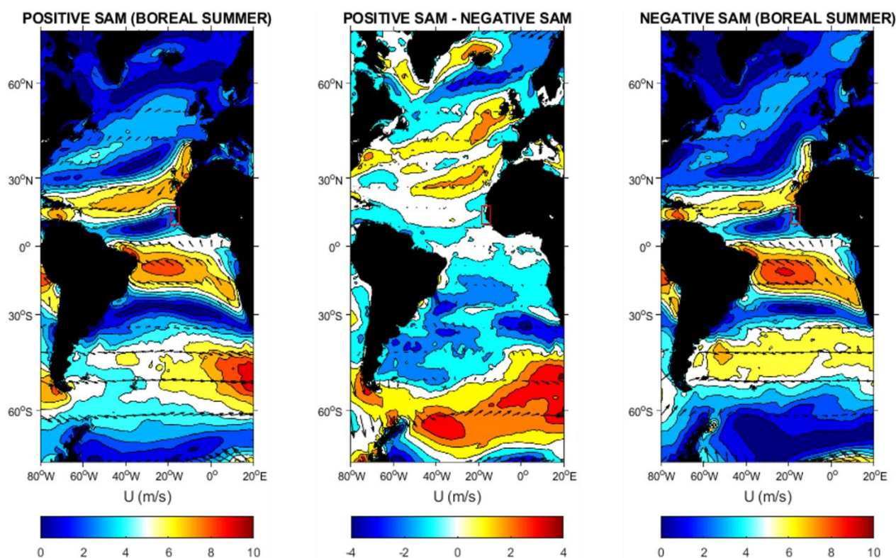
Figure 13. Average Wind speed in tropical Atlantic corresponding respectively to periods of maximum (+SAM, left) and minimum (-SAM, right) phases of SAM during boreal Summer, the wind spatial difference is shown on the middle panel, the Senegalese Coast is indicated by the red rectangle.
