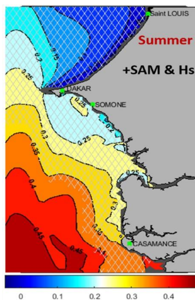
Figure 12. Spatial correlations between +SAM index and Hs during boreal Summer, computed on the Senegalese coast from 1980-2021, crosslines on maps indicated not significant areas (at 95% confidence interval, Mann Kendall Test).
